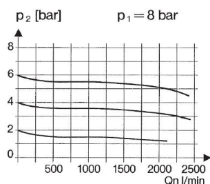
Diagram pretoka
