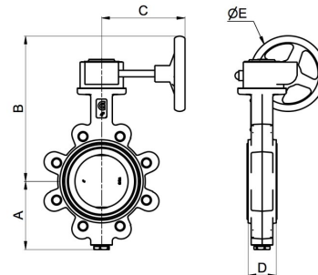
Flanged version
